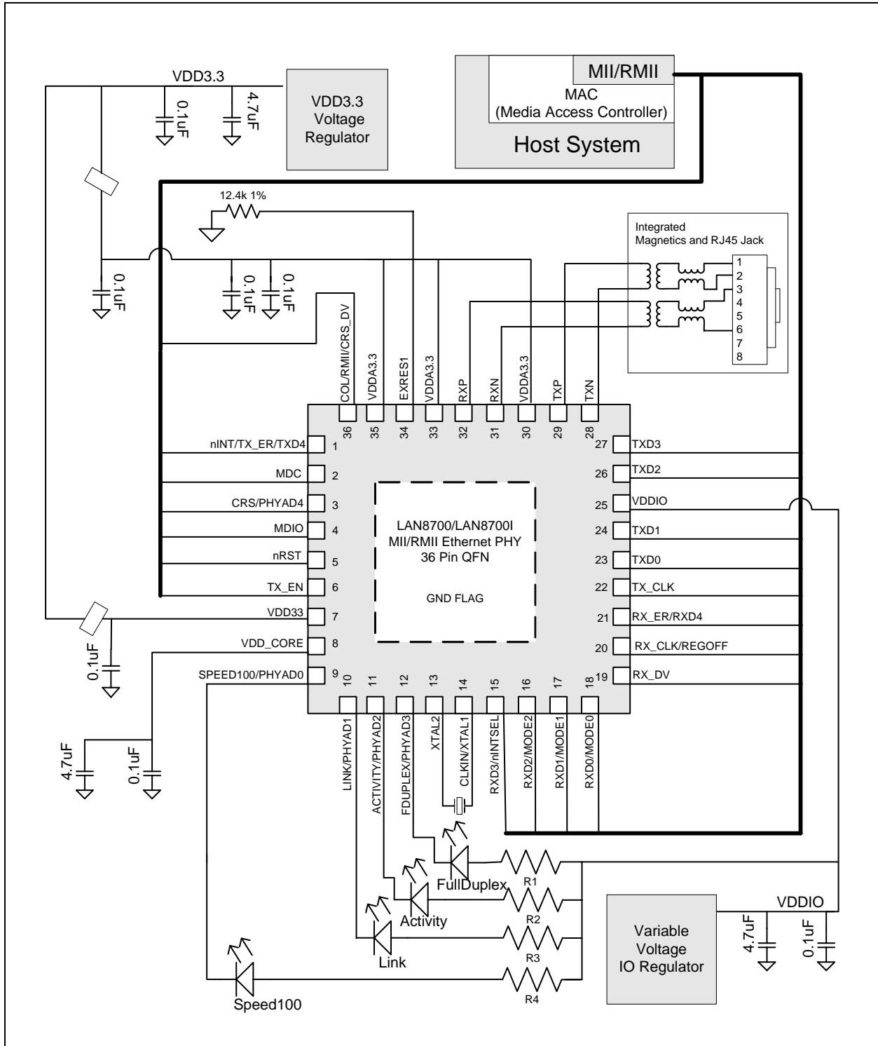
Figure 8.1 Simplified Application Diagram (see Section 8.4, "Reference Designs")
